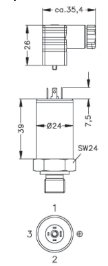
Micro, contact distance 9.4 mm (IP 65)
