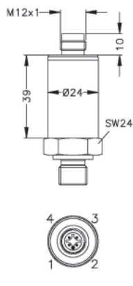
M12x1, 4-pin (IP 67)
