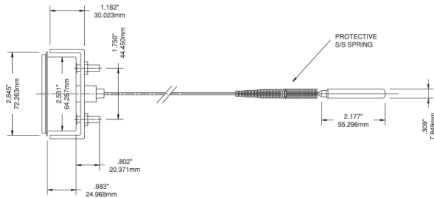
2.5" with U-Clamp
