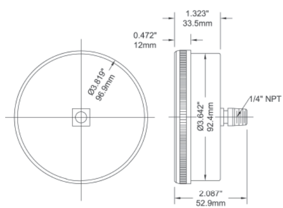
3.5" Back Connection
