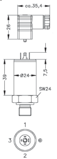
Micro, contact distance 9.4 mm (IP 65)
