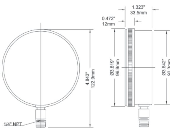
3.5" Bottom Connection
