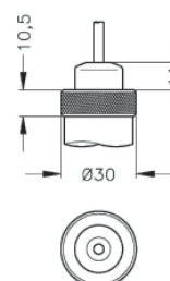
Cable outlet (IP 68) 5 Different cable types/lengths available
